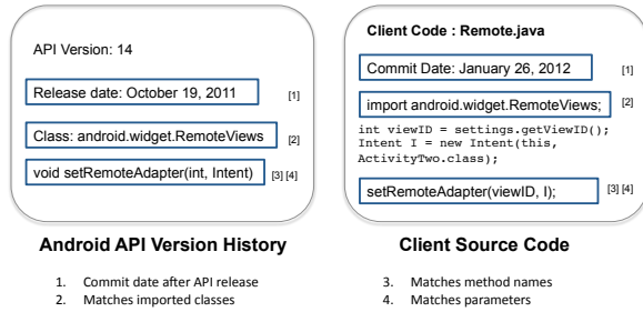
Figure 2. Identifying Android References in Client Source Code
